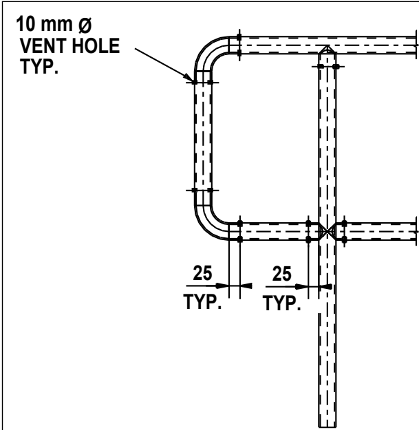
TYPICAL VENT HOLE DETAIL
