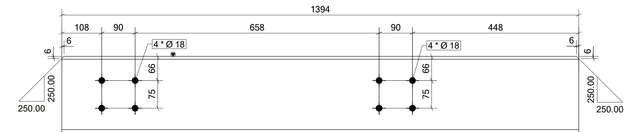
DETAIL OF FR002
